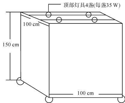
图 1 丝织品染料常规光老化实验装置示意 Fig. 1 Routine light aging experiment device of silk dyes
