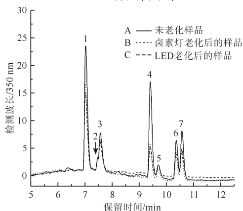
图 4 槐米在不同光源光老化 360 d 后的高效液相色谱图 Fig. 4 HPLC figure for pagoda tree after light aging for 360 days under different light sources
