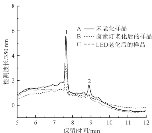
图 6 苏木在不同光源光老化 360 d 后的高效液相色谱图 Fig. 6 HPLC figure for spanwood after light aging for 360 days under different light sources
